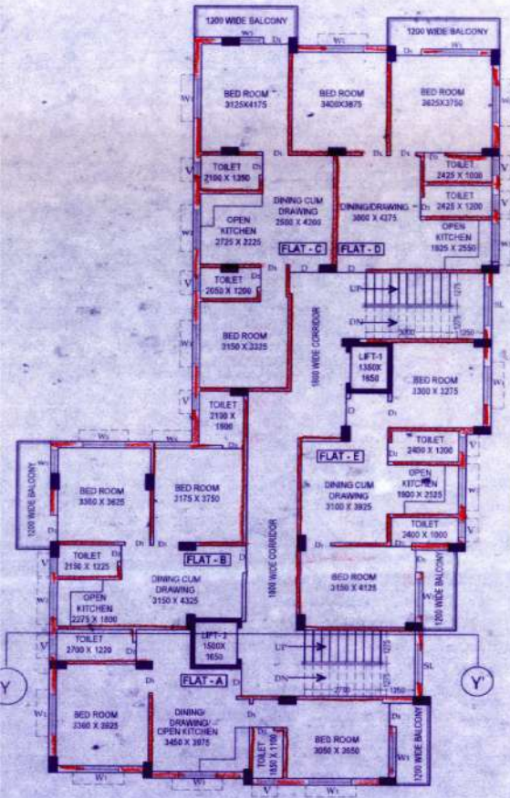
TYPICAL FLOOR PLAN (1ST & 2ND. FLOOR) ALREADY SANCTIONED VIDE PERMIT NO.-SWS-CBPAS/1606/2024/0524 SANCTIONED DATE: SCALE: (1:100)
