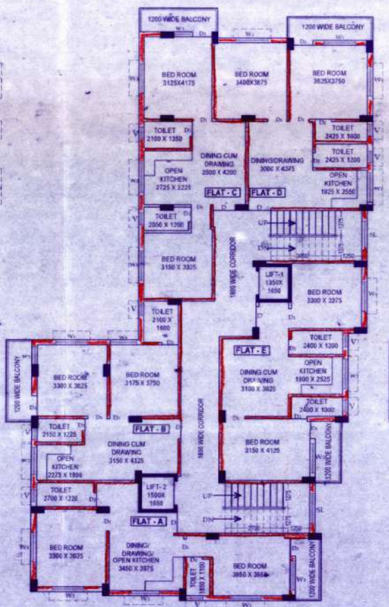
PROPOSED TYPICAL FLOOR PLAN (7TH, 8TH & 9TH. FLOOR PLAN) SCALE: (1:100)
