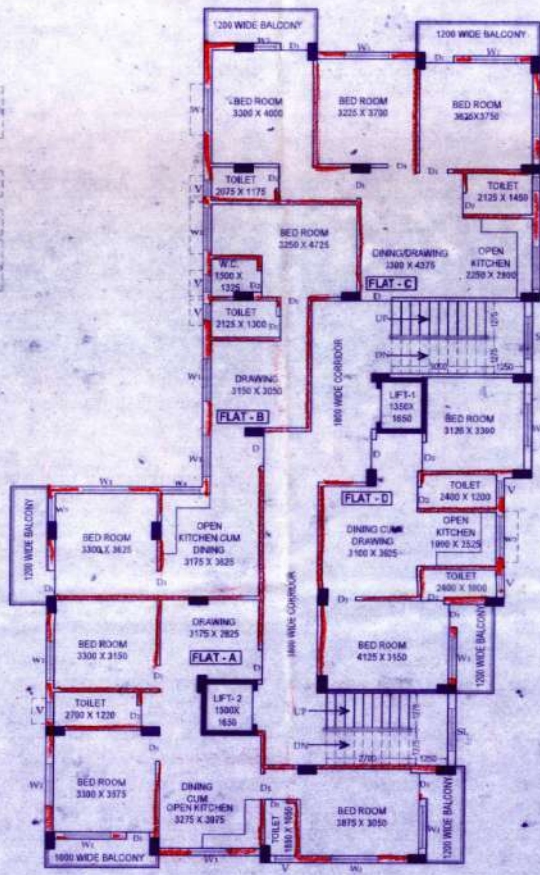
TYPICAL FLOOR PLAN (3RD & 4TH. FLOOR) ALREADY SANCTIONED VIDE PERMIT NO.-SWS-CBPAS/1606/2024/0524 SANCTIONED DATE: SCALE: (1:100)
