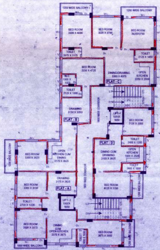
PROPOSED TYPICAL FLOOR PLAN (5TH & 6TH. FLOOR PLAN) SCALE: (1:100)
